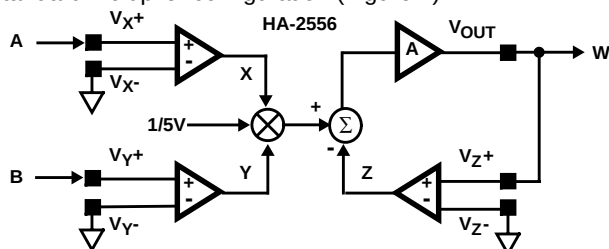
FIGURE 2. MULTIPLIER
