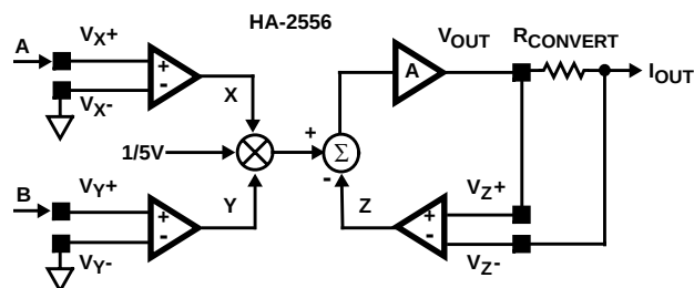
FIGURE 10. CURRENT OUTPUT
