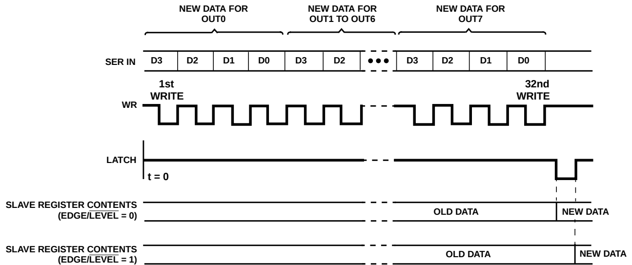
FIGURE 5. SERIAL PROGRAMMING MODE OPERATION ( SER/\overline{PAR} = 1 )
