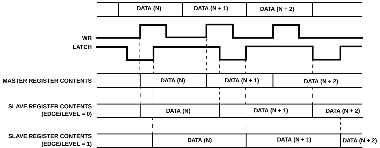
FIGURE 4. PARALLEL PROGRAMMING MODE OPERATION ( SER/\overline{PAR} = 0 )
