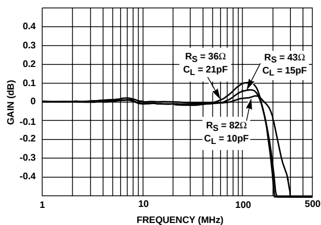
FIGURE 6. GAIN FLATNESS
