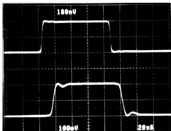
FIGURE 5. SMALL SIGNAL RESPONSE
