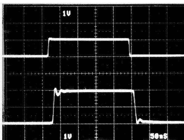
FIGURE 6. LARGE SIGNAL RESPONSE
