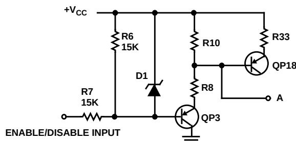
FIGURE 38. SIMPLIFIED SCHEMATIC OF ENABLE/DISABLE FUNCTION
