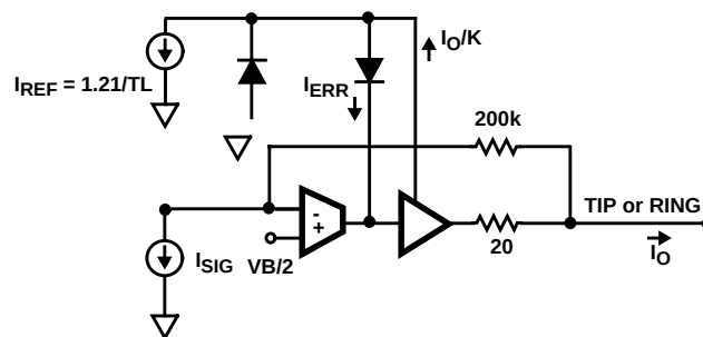
FIGURE 1. CURRENT LIMIT FUNCTIONAL DIAGRAM
