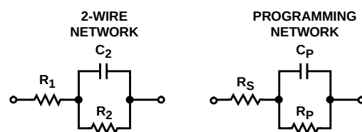
FIGURE 2. COMPLEX PROGRAMMING NETWORK
