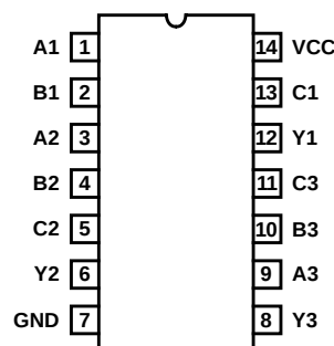
14 LEAD CERAMIC METAL SEAL FLATPACK PACKAGE (FLATPACK) MIL-STD-183S CDFP3-F14, LEAD FINISH C TOP VIEW
