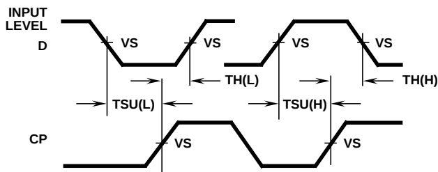
FIGURE 3. DATA SET-UP AND HOLD TIMES
