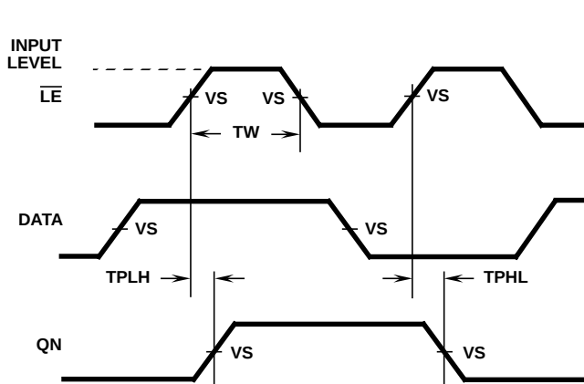
FIGURE 1. LATCH ENABLE PROPAGATION DELAYS
