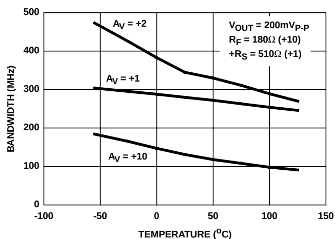
FIGURE 18. -3dB BANDWIDTH vs TEMPERATURE
