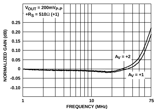
FIGURE 19. GAIN FLATNESS
