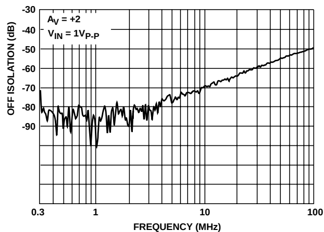
FIGURE 20. OFF ISOLATION
