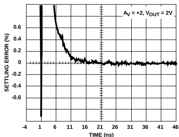
FIGURE 14. SETTLING RESPONSE
