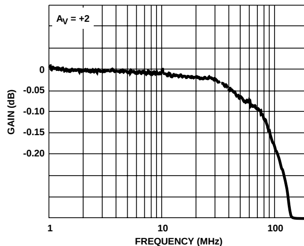
FIGURE 12. GAIN FLATNESS
