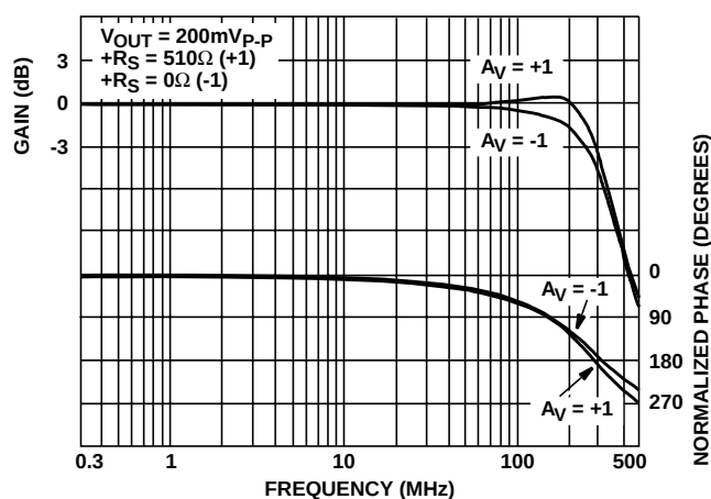
FIGURE 12. FREQUENCY RESPONSE
