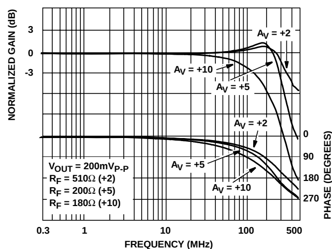
FIGURE 13. FREQUENCY RESPONSE
