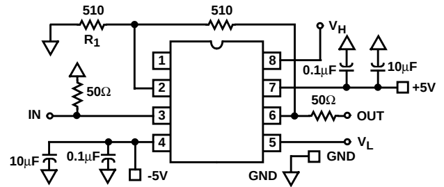
FIGURE 2C. SCHEMATIC
