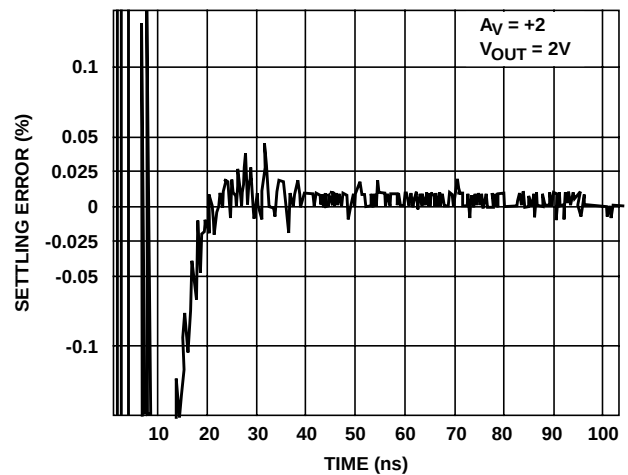
FIGURE 25. SETTLING RESPONSE
