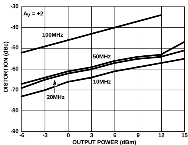
FIGURE 16. 2nd HARMONIC DISTORTION vs P_{\text{OUT}}
