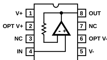
HFA1110/883 (CERDIP) TOP VIEW
