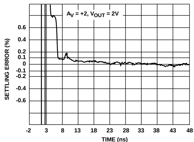
FIGURE 20. SETTLING RESPONSE
