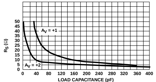
FIGURE 1. RECOMMENDED SERIES OUTPUT RESISTOR vs LOAD CAPACITANCE
