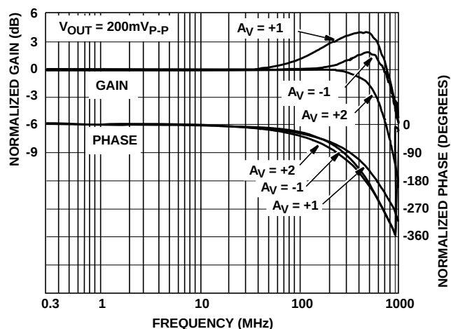
FIGURE 9. FREQUENCY RESPONSE
