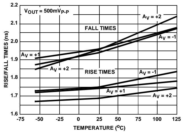
FIGURE 35. RISE AND FALL TIMES vs TEMPERATURE
