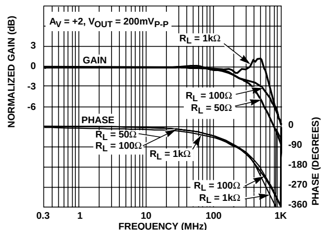
FIGURE 6. FREQUENCY RESPONSE FOR VARIOUS LOAD RESISTORS
