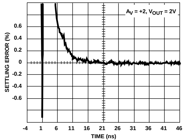
FIGURE 14. SETTLING RESPONSE
