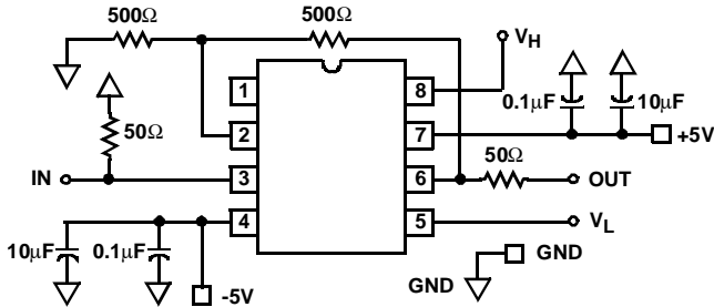
FIGURE 2. BOARD SCHEMATIC
