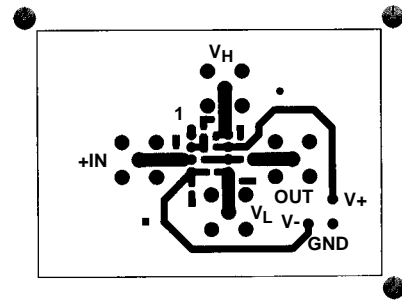
BOTTOM LAYOUT
