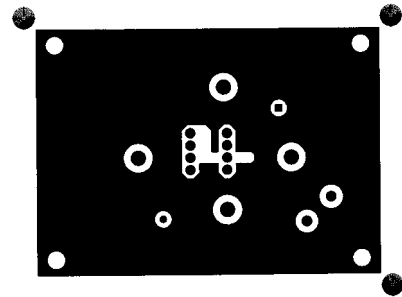
BOTTOM LAYOUT
