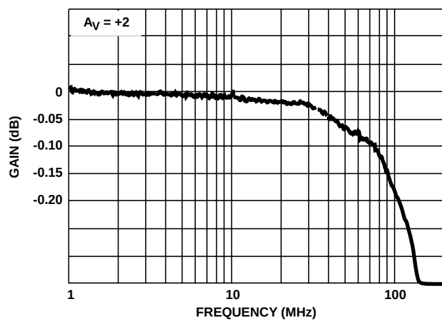
FIGURE 15. GAIN FLATNESS
