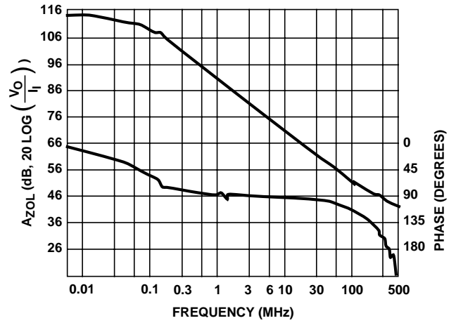
FIGURE 16. OPEN LOOP TRANSIMPEDANCE
