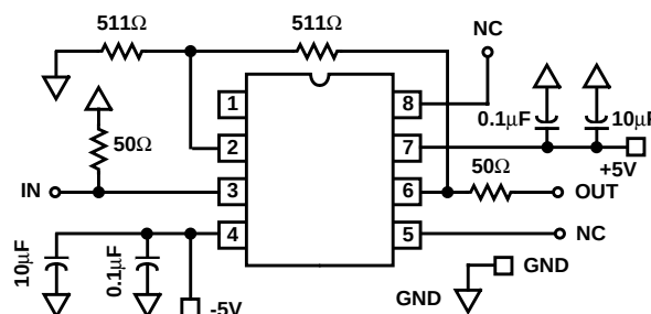
FIGURE 2. HFA11XXEVAL SCHEMATIC
