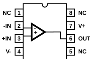
HFA1150 (SOIC) TOP VIEW
