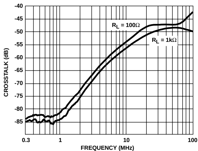
FIGURE 29. CROSSTALK
