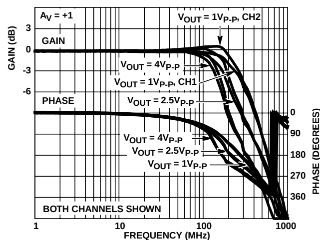
FIGURE 25. FREQUENCY RESPONSE FOR VARIOUS OUTPUT VOLTAGES
