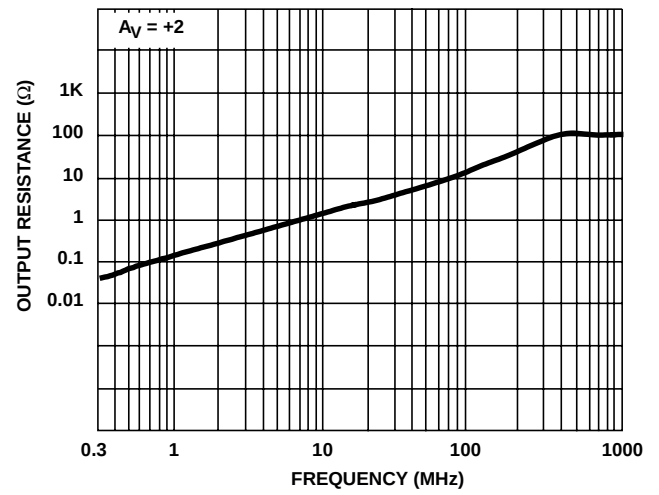
FIGURE 31. OUTPUT RESISTANCE
