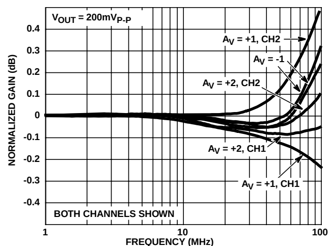
FIGURE 28. GAIN FLATNESS
