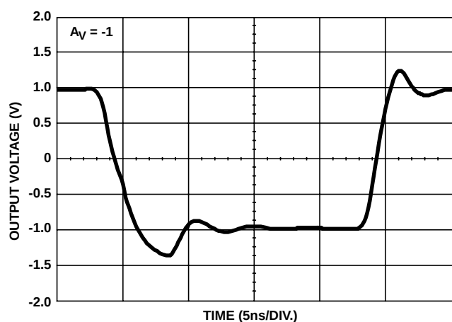
FIGURE 12. LARGE SIGNAL BIPOLAR PULSE RESPONSE
