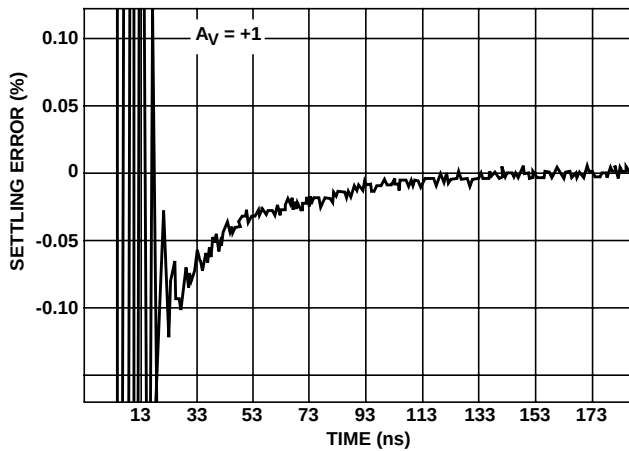
FIGURE 20. SETTLING RESPONSE
