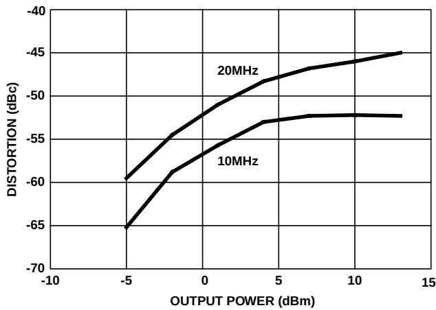
FIGURE 18. 2nd HARMONIC DISTORTION vs P_{\text{OUT}}
