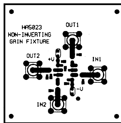
FIGURE 3A. TOP LAYOUT
