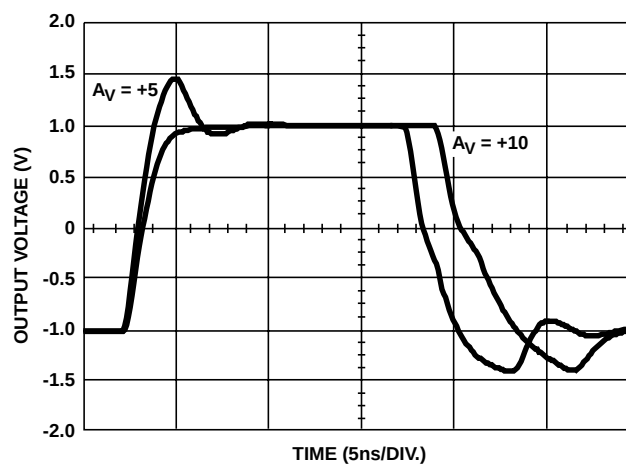
FIGURE 19. LARGE SIGNAL BIPOLAR PULSE RESPONSE
