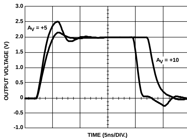
FIGURE 17. LARGE SIGNAL POSITIVE PULSE RESPONSE
