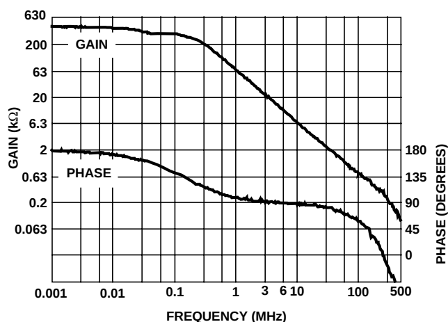
FIGURE 21. OPEN LOOP TRANSIMPEDANCE
