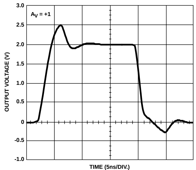
FIGURE 9. LARGE SIGNAL POSITIVE PULSE RESPONSE
