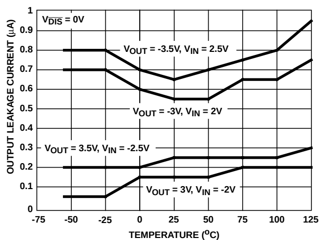
FIGURE 39. DISABLED OUTPUT LEAKAGE vs TEMPERATURE
