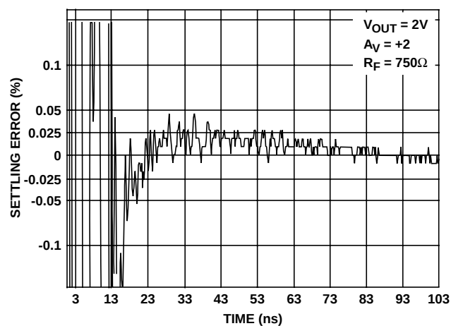
FIGURE 35. SETTLING TIME RESPONSE
