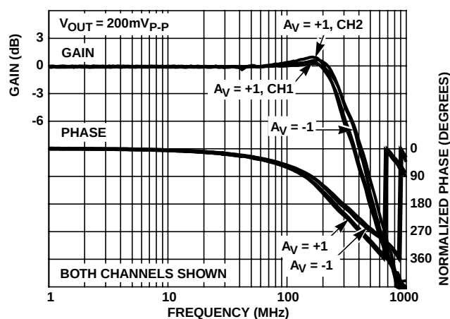
FIGURE 22. FREQUENCY RESPONSE
