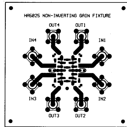
TOP LAYOUT
