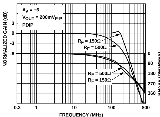
FIGURE 27. FREQUENCY RESPONSE
