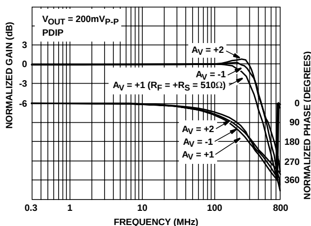
FIGURE 26. FREQUENCY RESPONSE
