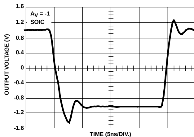
FIGURE 9. LARGE SIGNAL PULSE RESPONSE
