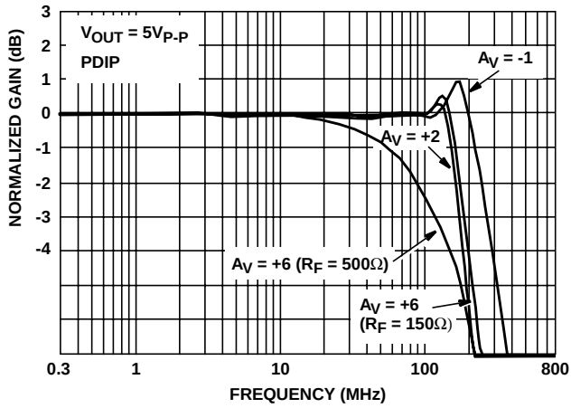
FIGURE 28. FULL POWER BANDWIDTH
