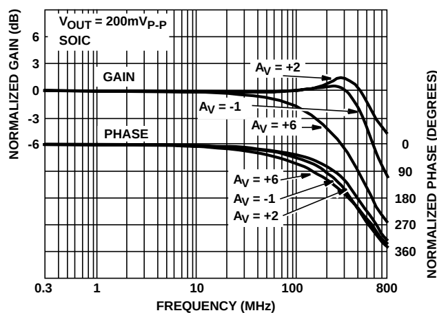
FIGURE 12. FREQUENCY RESPONSE
