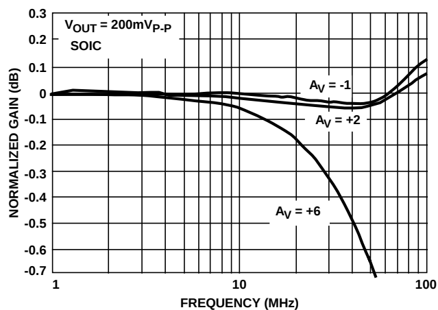
FIGURE 14. GAIN FLATNESS
