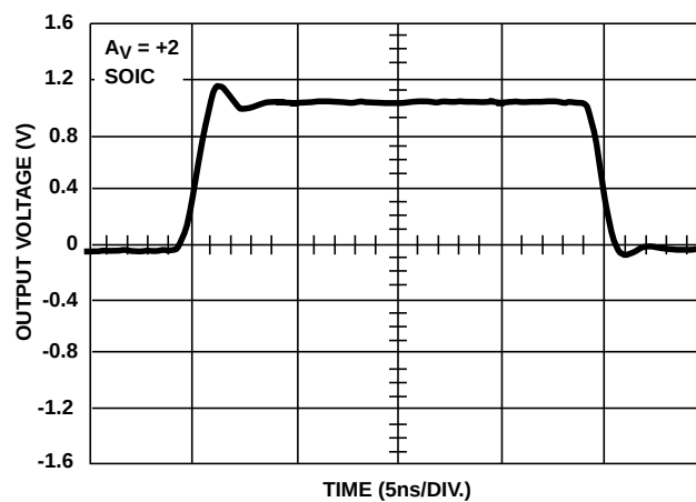
FIGURE 5. LARGE SIGNAL PULSE RESPONSE
