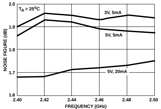
FIGURE 3. NOISE FIGURE vs FREQUENCY
