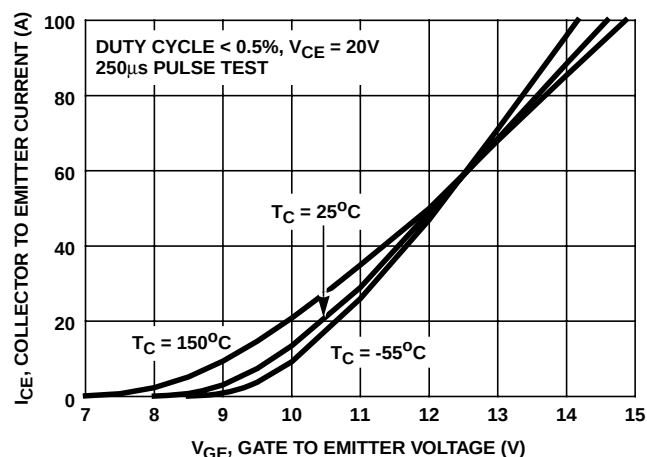
FIGURE 13. TRANSFER CHARACTERISTIC
