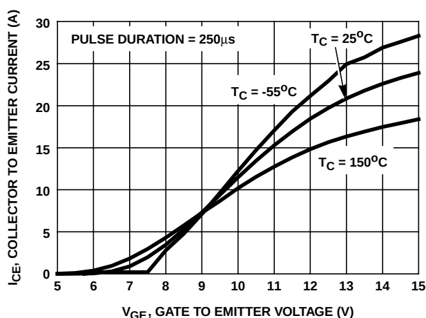
FIGURE 13. TRANSFER CHARACTERISTIC
