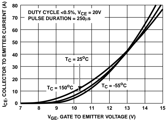
FIGURE 13. TRANSFER CHARACTERISTICS
