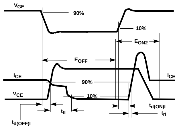
FIGURE 19. SWITCHING TEST WAVEFORMS
