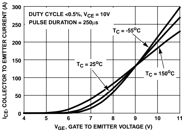
FIGURE 13. TRANSFER CHARACTERISTIC
