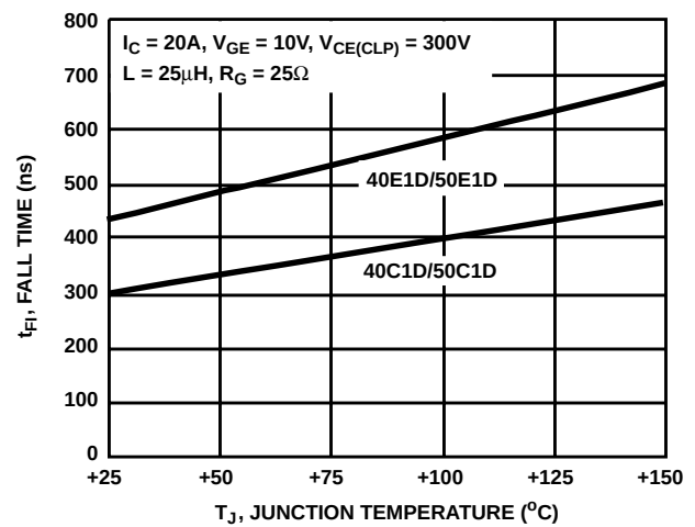
FIGURE 12. TYPICAL FALL TIME ( I_C = 20\text{A} )
