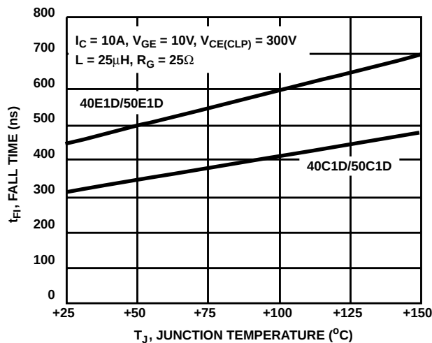
FIGURE 11. TYPICAL FALL TIME ( I_C = 10\text{A} )
