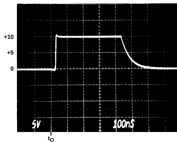
FIGURE 2B. V_{IN} = +10V
