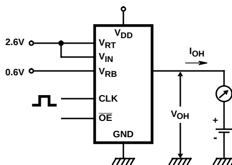
FIGURE 25. DIGITAL OUTPUT CURRENT TEST CIRCUIT
