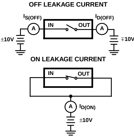
FIGURE 2B. TEST CIRCUITS
