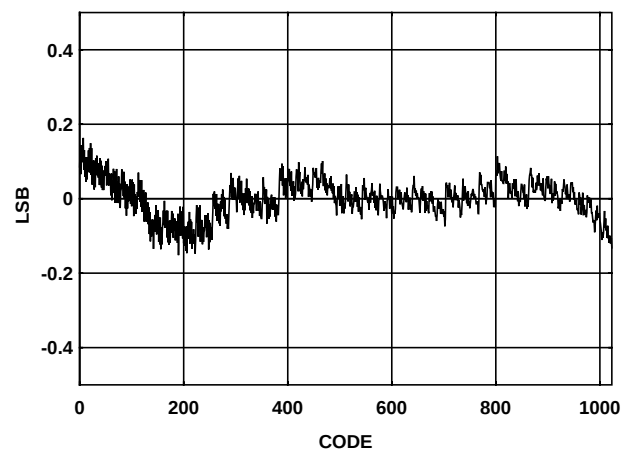
FIGURE 18. INTEGRAL NONLINEARITY
