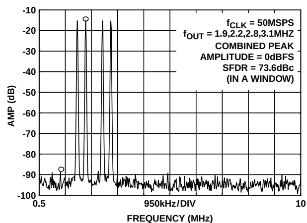
FIGURE 16. FOUR-TONE, CLOCK = 50MSPS
