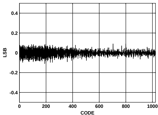
FIGURE 17. DIFFERENTIAL NONLINEARITY
