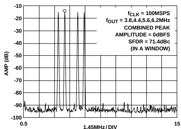
FIGURE 14. FOUR-TONE, CLOCK = 100MSPS
