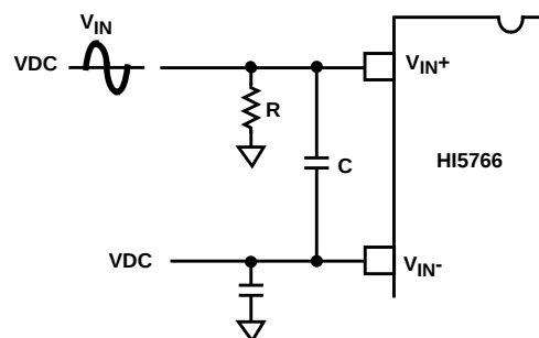
FIGURE 28. DC COUPLED SINGLE ENDED INPUT
