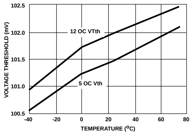
FIGURE 10. OC VOLTAGE THRESHOLD WITH R_{LIM} = 10k\Omega
