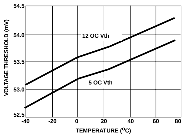
FIGURE 9. OC VOLTAGE THRESHOLD WITH R_{LIM} = 5k\Omega
