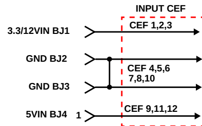
BUS BOARD
