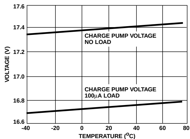
FIGURE 8. PUMP VOLTAGE
