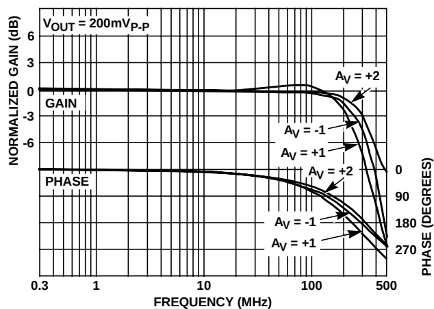
FIGURE 10. FREQUENCY RESPONSE
