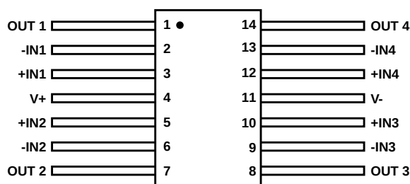
HS9-5104ARH-T (FLATPACK), CDFP3-F14 TOP VIEW
