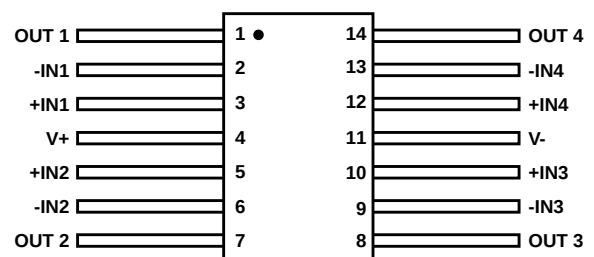
HS-5104ARH (FLATPACK) CDFP3-F14 TOP VIEW
