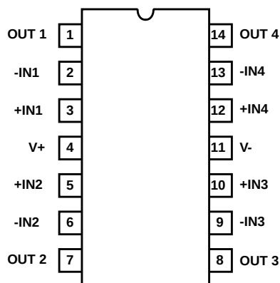
HS-5104ARH (SBDIP) CDIP2-T14 TOP VIEW
