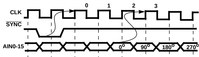
FIGURE 15B. DATA FLOW DIAGRAM FOR DOWN CONVERT AND DECIMATE MODE ( \overline{\text{INT/EXT}} = 0 )
