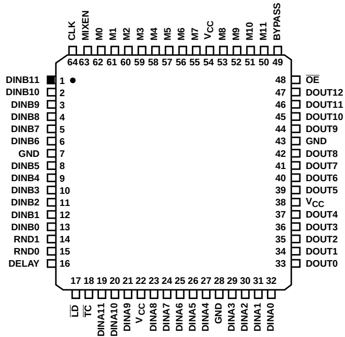
64 LEAD MQFP TOP VIEW
