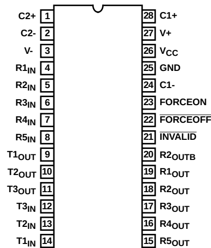
ICL3244 (SOIC, SSOP) TOP VIEW
