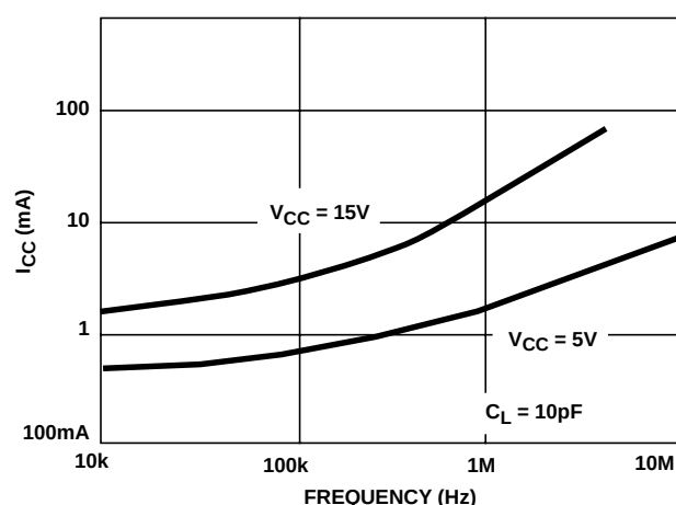
FIGURE 6. NO LOAD I_{CC} vs FREQUENCY
