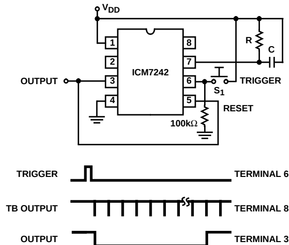
FIGURE 4. MONOSTABLE OPERATION
