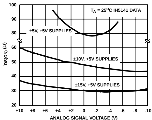
FIGURE 2. r_{DS(ON)} vs POWER SUPPLIES
