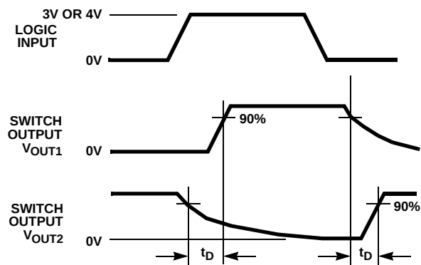
FIGURE 3A. MEASUREMENT POINTS (ISL5122 ONLY)
