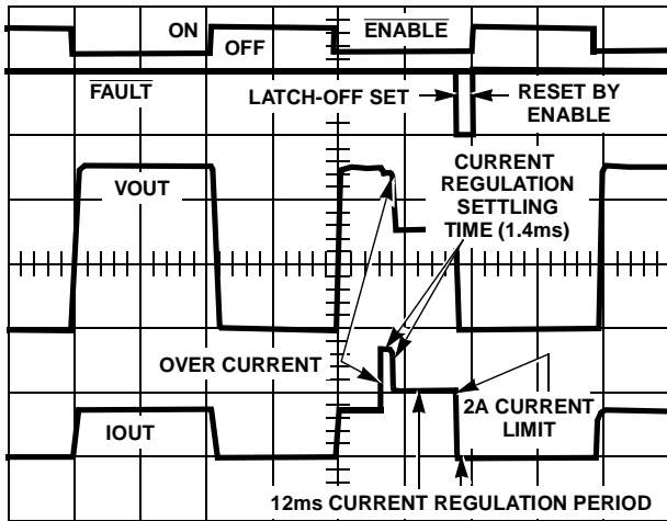
FIGURE 2. OPERATIONAL WAVEFORMS
