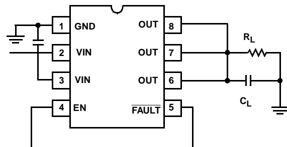
FIGURE 1. ISL6121 TYPICAL APPLICATION
