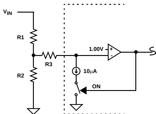
FIGURE 5. UV HYSTERESIS
